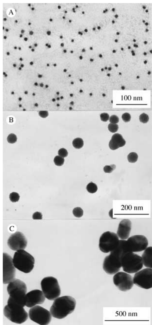
Figure 3. TEM images of Au nanoparticles enlarged by 0.01 % \text{HAuCl}_4 and 0.4 mM \text{NH}_2\text{OH} \cdot \text{HCl} in aqueous solution. A) Seeds, B) after one treatment for 2 min, C) after two treatments each of 2 min.
